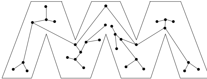
Fig. 12. Drawing of a 31-node complete binary tree by our algorithm inside a NM-shaped polygon
