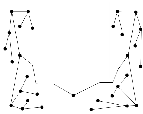
Fig. 8. Drawing of a 31-node complete binary tree by our algorithm inside a U-shaped rectilinear polygon
