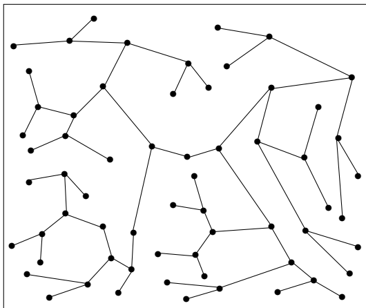
Fig. 6. Drawing of a 63-node complete binary tree by our algorithm inside a square
